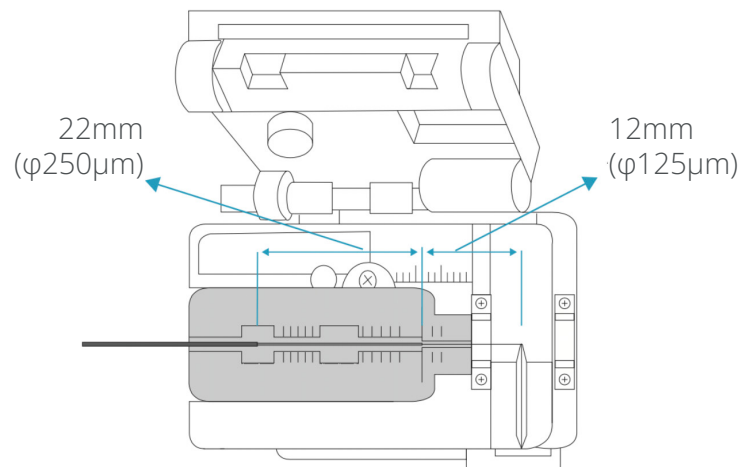
Cleaver
